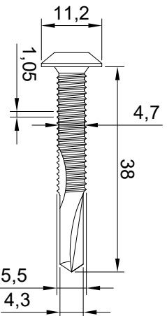
TSLP5.5-38-5 Scale 1:1
