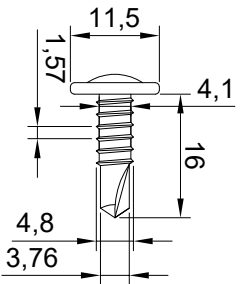
TSLP4.8-16-3 Scale 1:1
