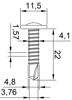
TSLP4.8-22-3 Scale 1:1
