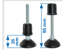
Height-adjustable foot plate available as a safety accessory
