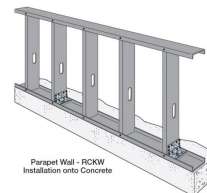
RCKW - Parapet Wall
