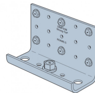
RCKW5.5 Fastener Pattern 3 - Concrete Application
