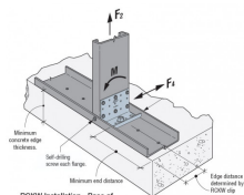
RCKW - Concrete Support
