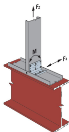
RCKW - Steel Support
