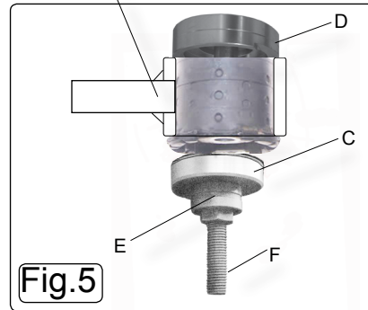
Composite section through housing boss (4 places)
